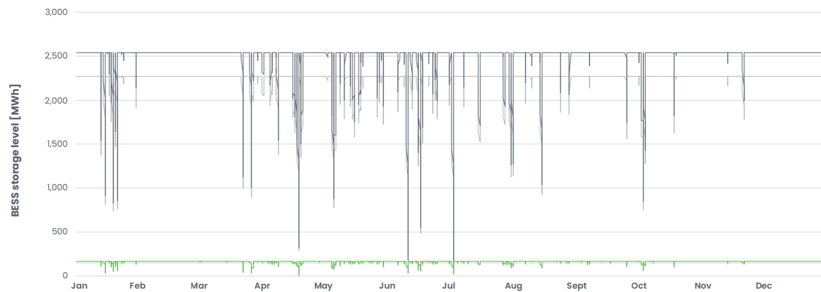
Figure 16: Required storage capacity for BESS-backup solution – case study Namibia
