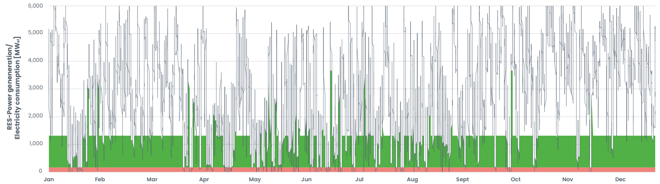
Figure 12: Electricity consumption for H 2 production and Haber Bosch process (including air separation, compression, reactor and ammonia cooling) – case study Namibia
