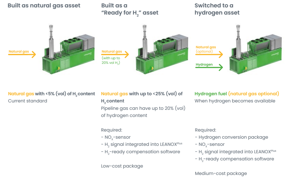
Figure 7: Demand-oriented conversion of INNIO Group's Jenbacher engines to hydrogen operation
